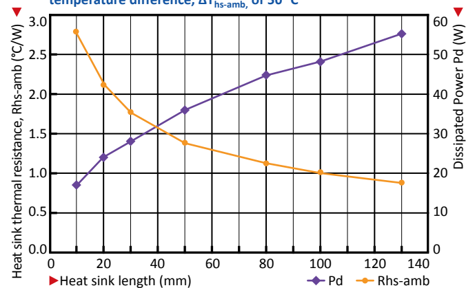
ModuLED performance data at a heat sink to ambient temperature difference, \Delta T_{hs-amb} , of 50 °C
