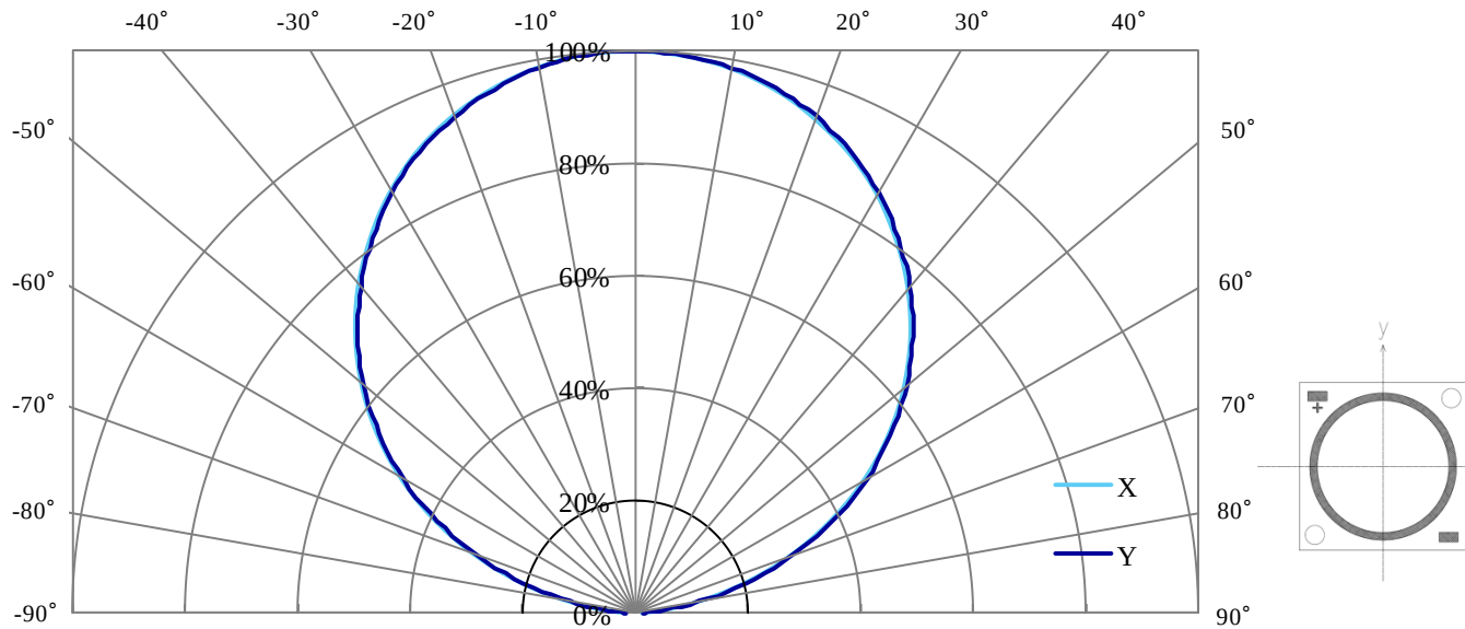
Radiation Characteristic
