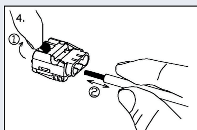
Connection and disconnection of flexible conductors by pushing the release lever
