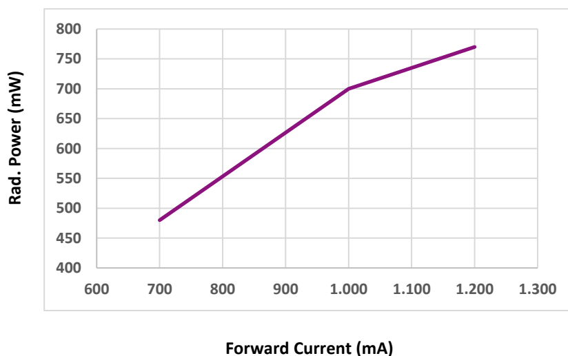
Rad. Power (mW) x Forward Current (mA) (Tj 50°C)
